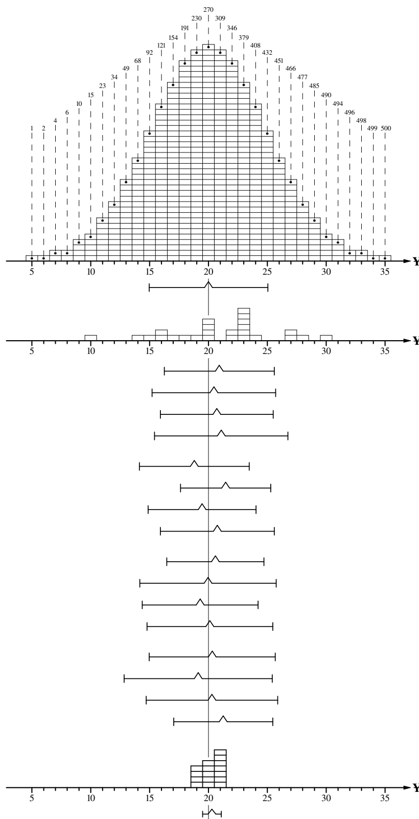
Figure 2.5a. EQUIPROBABLE SELECTING: Diagrammatic Illustration 1 of 3 Selecting from a ‘Normally’ Distributed Respondent Population
