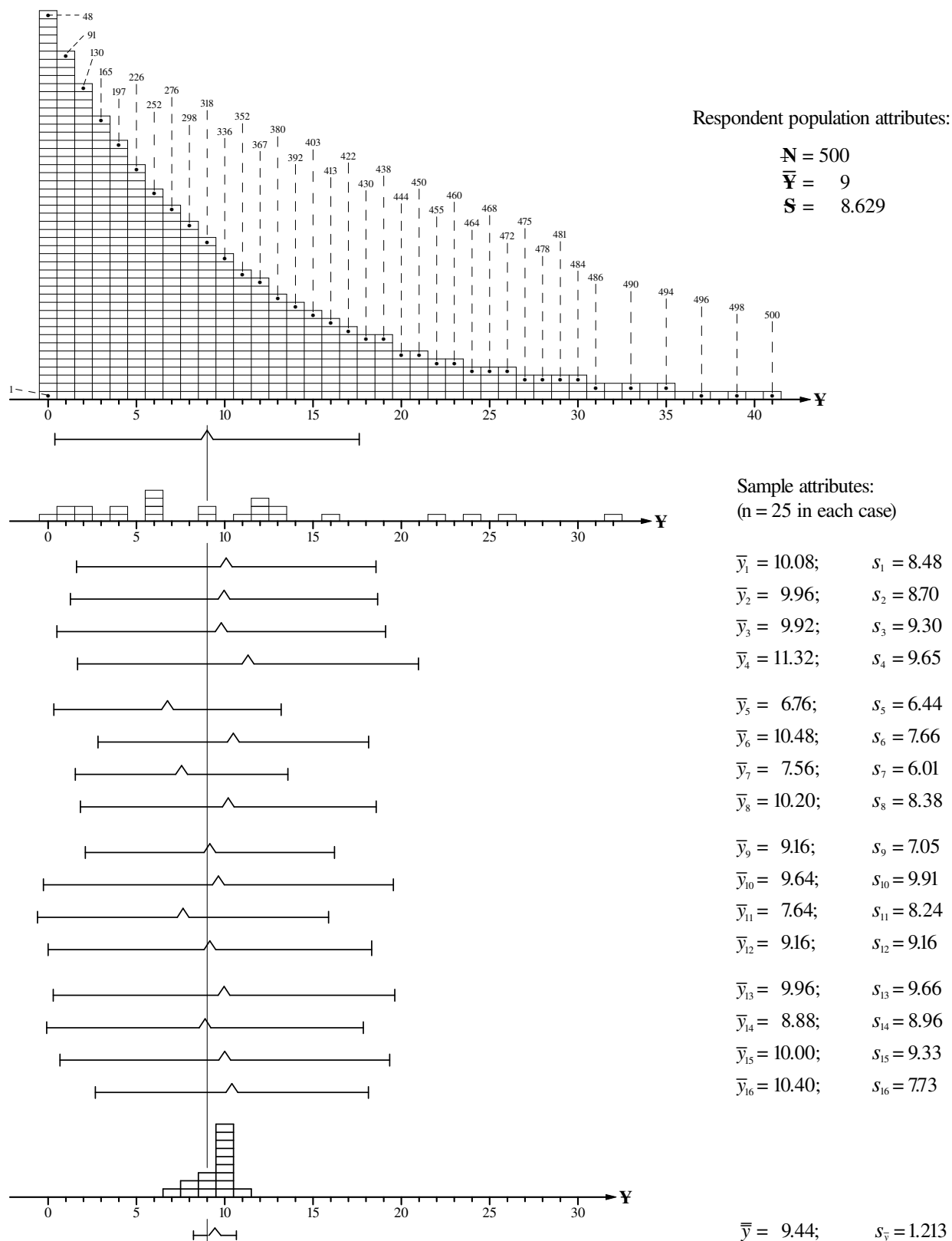
Figure 2.5c. EQUIPROBABLE SELECTING: Diagrammatic Illustration 3 of 3 Selecting from an ‘Exponentially’ Distributed Respondent Population
