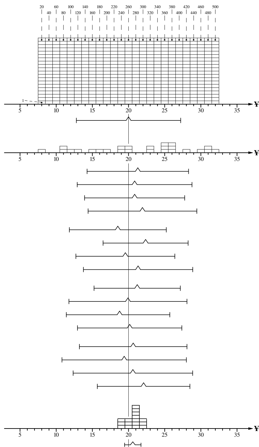
Figure 2.5b. EQUIPROBABLE SELECTING: Diagrammatic Illustration 2 of 3 Selecting from a ‘Uniformly’ Distributed Respondent Population
