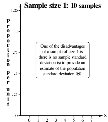
Figure 2.5f. SELECTING: Histograms of Sample Standard Deviations
