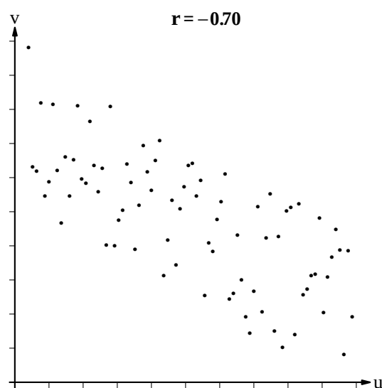
Figure 4.5c. CORRELATION: Scatter Diagrams ( n = 80 ) for Negative r -values (continued)
