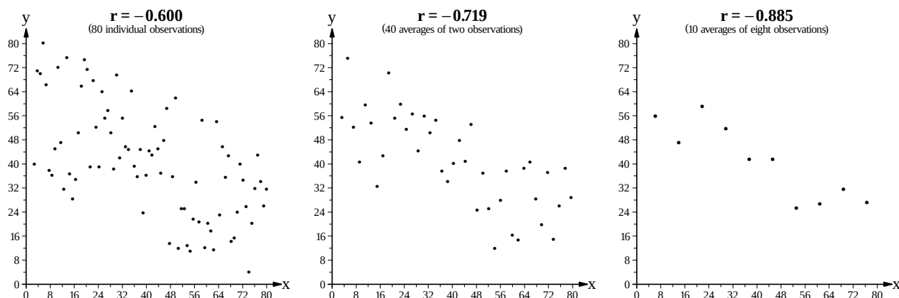
Figure 4.5. ANALYSIS STAGE: Correlation (continued 2)
