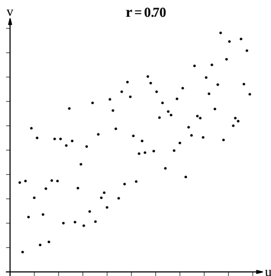
Figure 4.5a. CORRELATION: Scatter Diagrams ( n = 80 ) for Positive r -values (continued)
