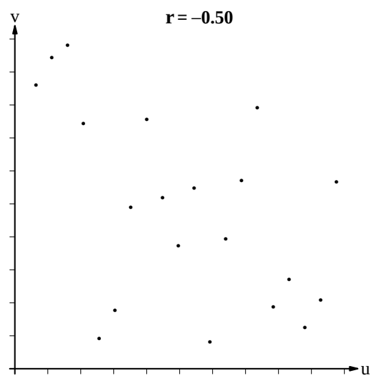
Figure 4.5b. CORRELATION: Scatter Diagrams ( n = 20 ) for Negative r -values
