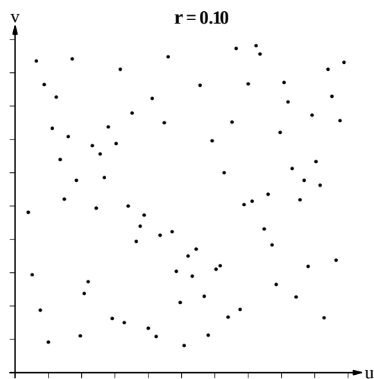
Figure 4.5a. CORRELATION: Scatter Diagrams ( n = 80 ) for Positive r -values
