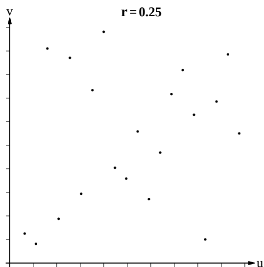
Figure 4.5b. CORRELATION: Scatter Diagrams ( n = 20 ) for Positive r -values (continued)
