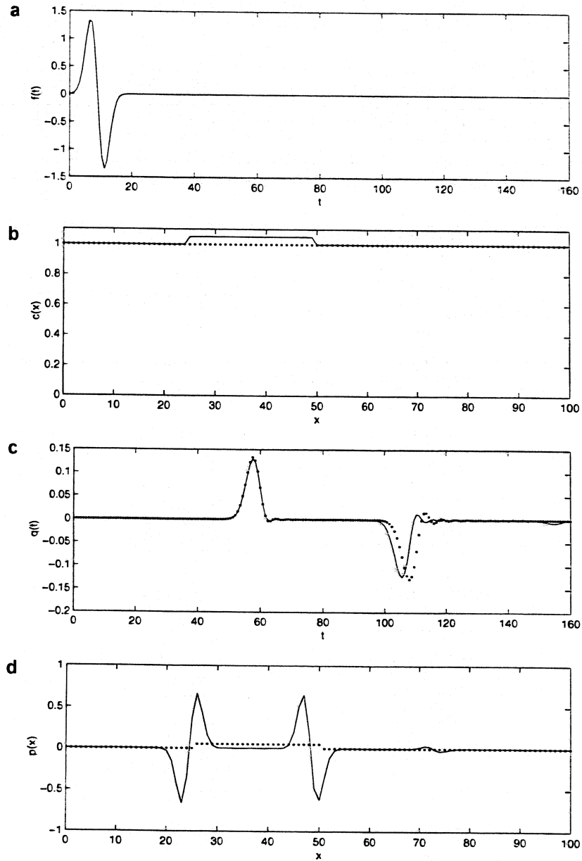
FIG. 4. (a) The excitation used in the examples. (b) The two sound speed profiles, c_1(x) in dots, c_2(x) in solid. (c) The graphs of (h_2 - h_1) and J(c_1)(c_2 - c_1) . (d) The graph of p = J(c_1)^2(h_2 - h_1) , shown for comparison, is the graph of c_2 - c_1 .
