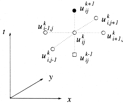
FIG. 3. The stencil for the 2-D problem for an interior node. Boundary and corner nodes are slightly different and require separate treatment.
