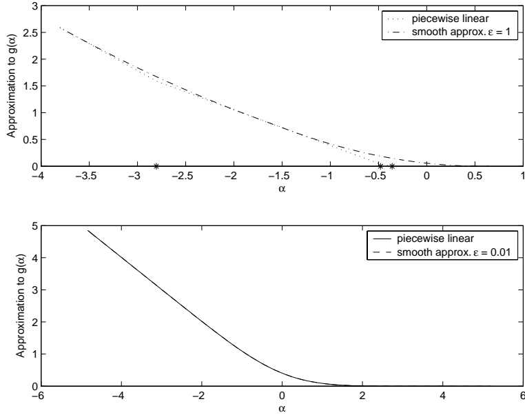
Figure 3: Approximations to g(\alpha) = \mathbf{E}([S - \alpha]^+)
