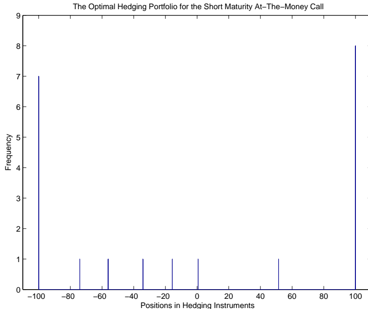
Figure 1: Histogram of Holdings of the Optimal Portfolio x_0^* From (18): \beta = 0.95
