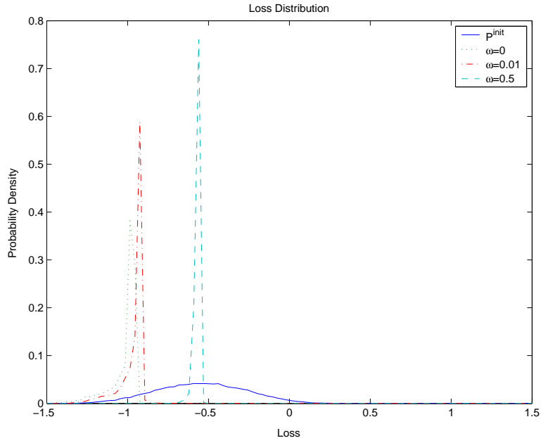
Figure 2: Loss Distributions of the Optimal Hedging Portfolios in Table 9
