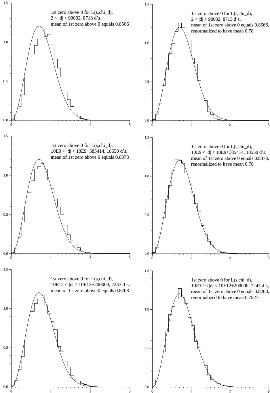
Figure 1.6: Distribution of the 1st zero above 0 for L(s, \chi_d) , as compared to \nu_1(\text{USp})(t) .
