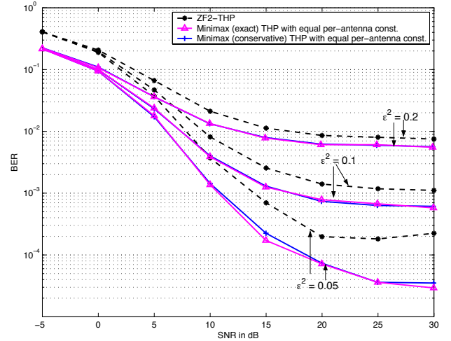
Fig. 7. Comparison between the performance of the exact and conservative minimax precoding methods with equal per-antenna constraints, and the ZF2-THP [3], [4], in the presence of uniformly distributed quantization errors with \epsilon^2 = 0.05, 0.1, 0.2 for a system with n_t = 4 and K = 3 , using QPSK signaling.
