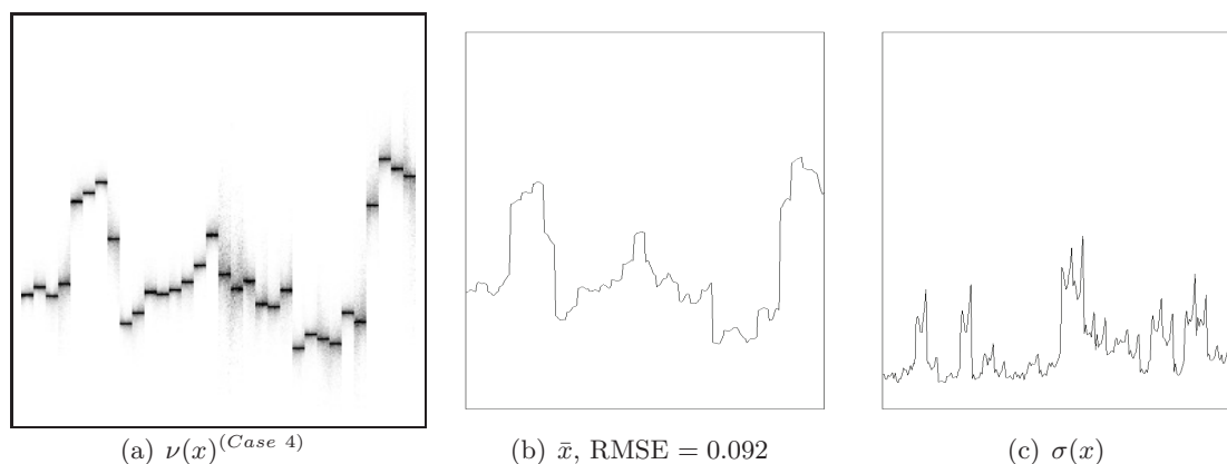
Figure 16. (a) Pictorial representation of measure \nu(x)^{(Case\ 4)} for the u(256, j) , 1 \leq j \leq 256 , row of pixels for the normalized Lena image plus Gaussian noise \sigma = 0.1 . (b) Mean values \bar{x} of \nu(x)^{(Case\ 4)} . (c) Variance \sigma(x) of this measure—vertical scale [0, 0.15] . In all cases, h = 0.1 . These figures complement the Case 1–3 results of Figure 8. 8 \times 8 -pixel range blocks, 16 \times 16 -pixel domain blocks.
