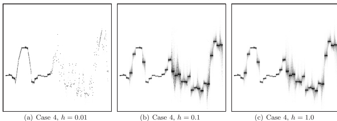
Figure 15. Pictorial representations of measures \nu(x)^{(Case\ 4)} for the u(256, j) , 1 \leq j \leq 256 , row of pixels of the Lena image. Three values of the weighting parameter h in (21) have been used, with P = 2 . These pictures complement the Case 1–3 results of Figure 7. 8 \times 8 -pixel range blocks, 16 \times 16 -pixel domain blocks.
