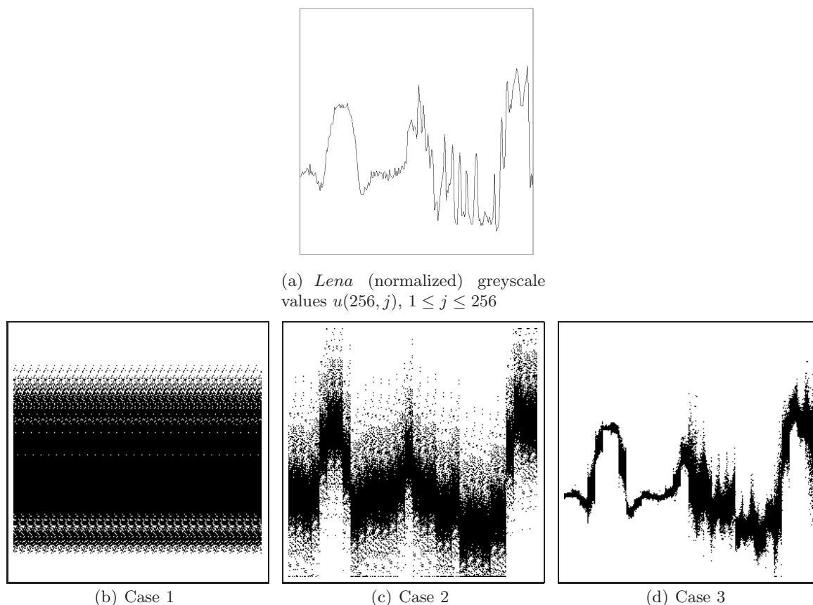
Figure 6. (a) Greyscale values of the normalized Lena image for the row of pixels u(256, j) , j = 1, \dots, 256 . (b)–(d) Pictorial representations of the contributions to the measures \nu(x)^{(Case\ q)} , q = 1, 2, 3 , respectively, for this row of pixels. The measures are arranged in vertical columns and occupy 256 bins that range in value from 0 (bottom) to 1 (top). In each case, the leftmost measure corresponds to j = 1 , and the rightmost to j = 256 .
