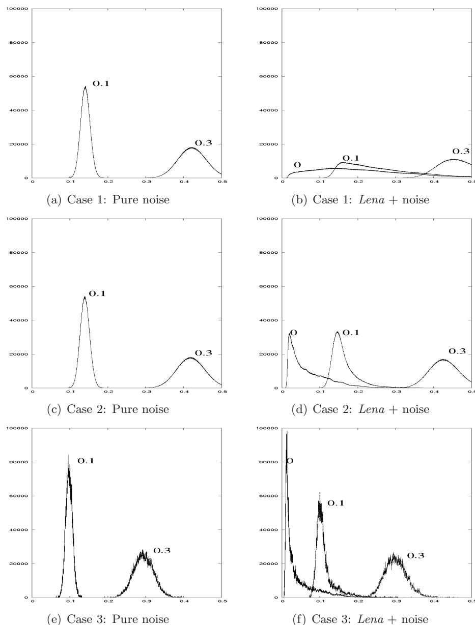
Figure 5. \Delta -error distributions for constant image u = 0.5 (left) and normalized Lena image (right) plus independent Gaussian noise \mathcal{N}(0, \sigma^2) , Cases 1–3. For \sigma = 0 , the \Delta -distributions of the image u = 0.5 consist of a single peak at \Delta = 0 .
