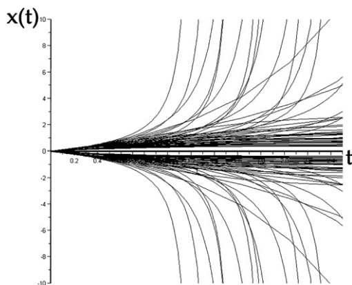
Fig. 1. Some selections of the integral inclusion x(t) \in (Tx)(t) = \int_0^t (P_0 + P_1 x(s) + P_2 x^2(s)) ds , where each P_i is the interval [-1, 1] .
