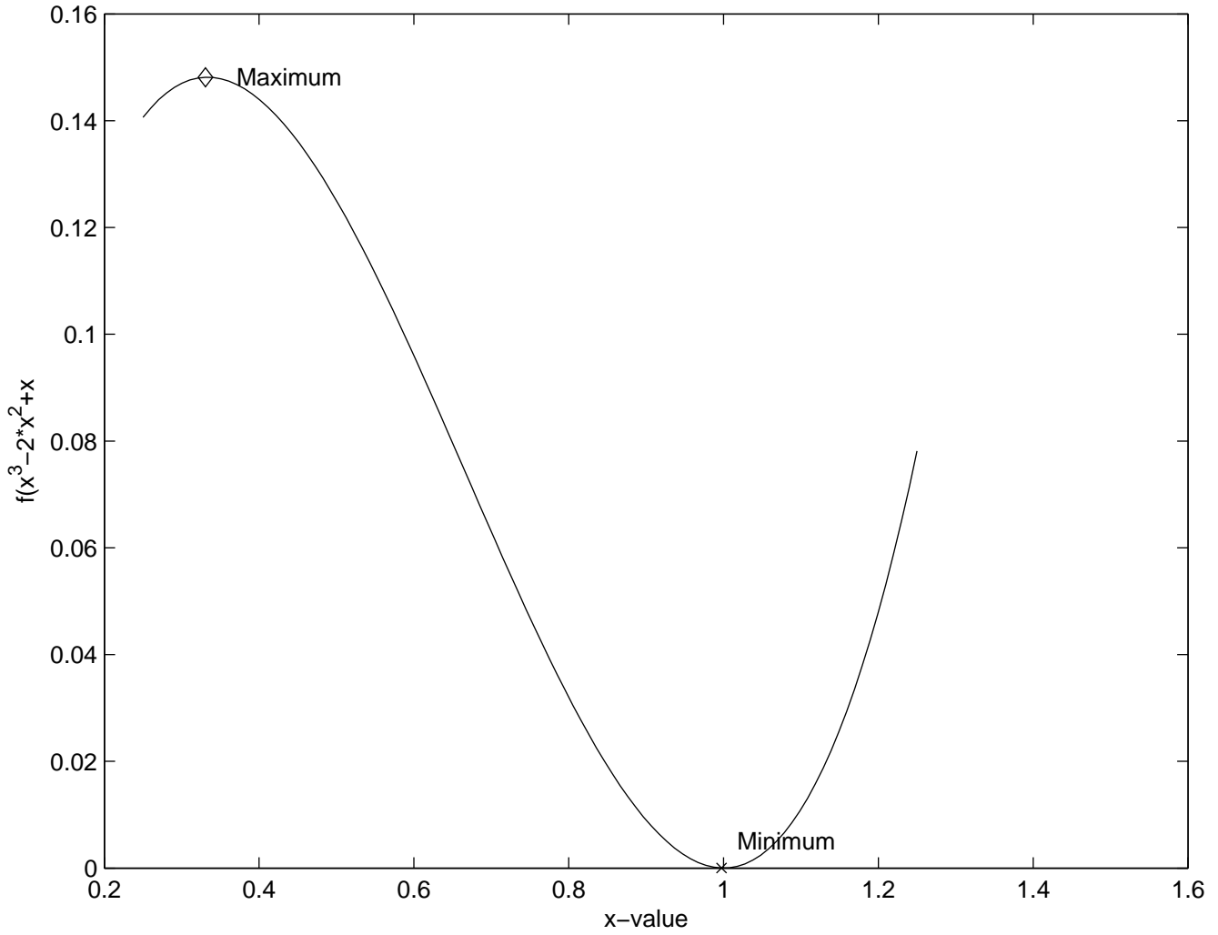
Find the Maximum and Minimum Using Discretization/Plotting
