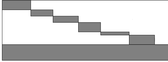
Figure 5.1: Sparsity Pattern of Matrix A
