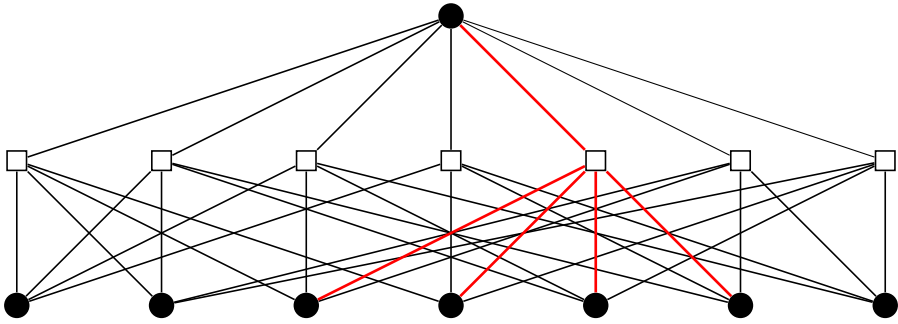
Fig. 5 Skutella’s example, which shows that the bidirected cut formulation and our new formulation both have a gap of at least \frac{8}{7} . The shaded edges denote one of the quasi-bipartite full components on 5 terminals
