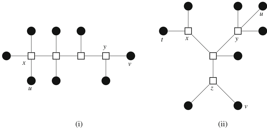
Fig. 4 The figure shows the two types of full components when b \leq 4 . On the left is a full component where the Steiner vertices form a path, and on the right is a full component where the Steiner vertices form a star with 3 tips
