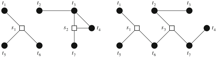
Fig. 2 Left a collection \mathcal{S} = \{t_1, t_5, t_6\}, \{t_3, t_4, t_7\}, \{t_2, t_3\}, \{t_3, t_4\} of 4 full components. Right a Steiner tree with \mathcal{S} -decomposition (\{t_1s_1, t_5s_1, t_6s_1, t_2t_3\}, \{t_2, t_6, t_7\}, \{t_4, t_7\})
