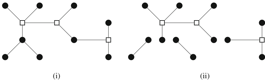
Fig. 1 The figure shows a Steiner tree in (i) and its decomposition into full components in (ii). Square and round vertices correspond to Steiner and terminal vertices, respectively. This particular tree is 5-restricted
