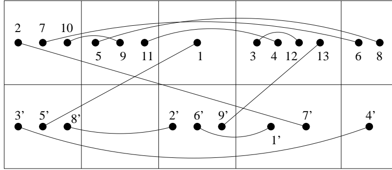
Figure 2: A labelled paired array.
