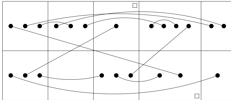
Figure 4: A paired array.
