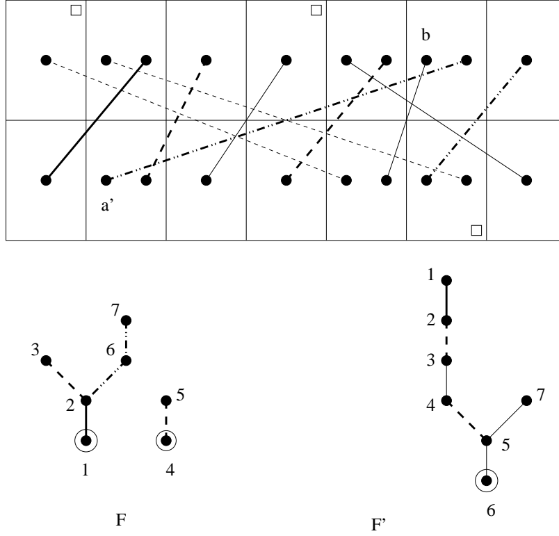
Figure 8: A vertical paired array with rightmost forests.
