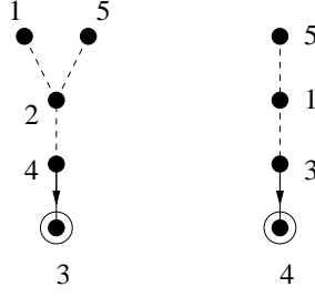
Figure 6: The rightmost trees for Figure 5.
