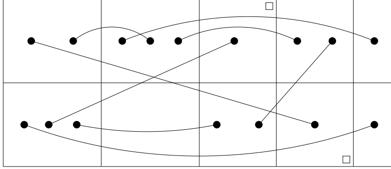
Figure 5: A minimal paired array.
