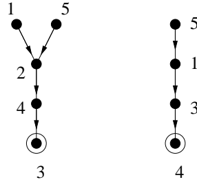
Figure 3: Two rooted trees.
