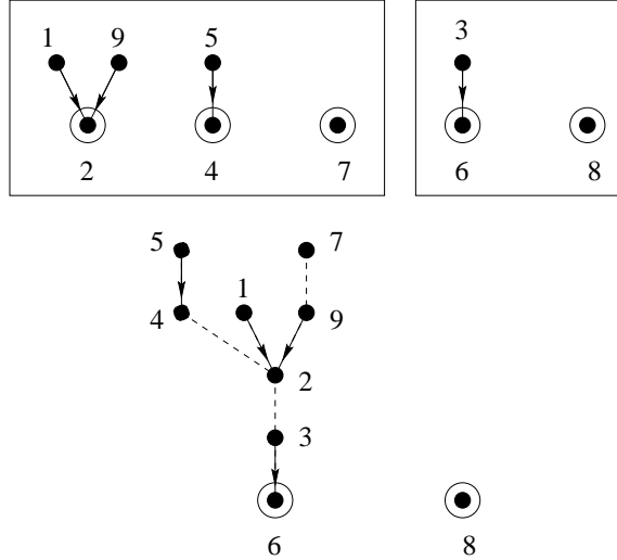
Figure 1: A rooted forest and subforest.
