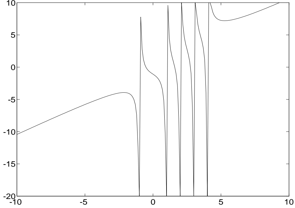
Figure 2: Secular antiderivative
