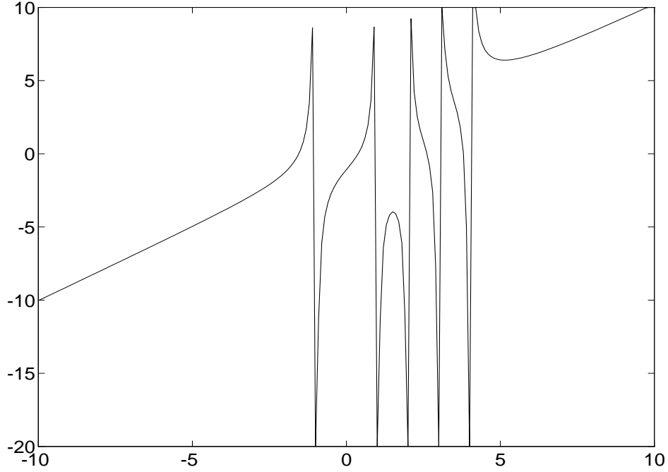
Figure 1: Secular antiderivative
